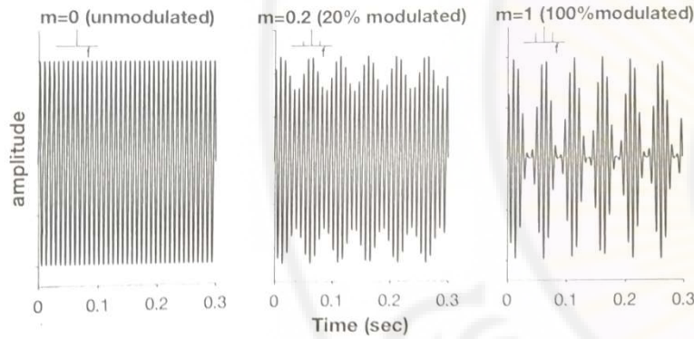
FIGURE 5-10. Waveforms of three different SAM tones at different modulation depths. Going from left to right, the stimuli progress from no modulation ( m = 0 ), 20% modulation ( m = 0.2 ) and fully modulated ( m = 1 ). The small insets in the upper left hand corners represent the spectra of the SAM tones.
