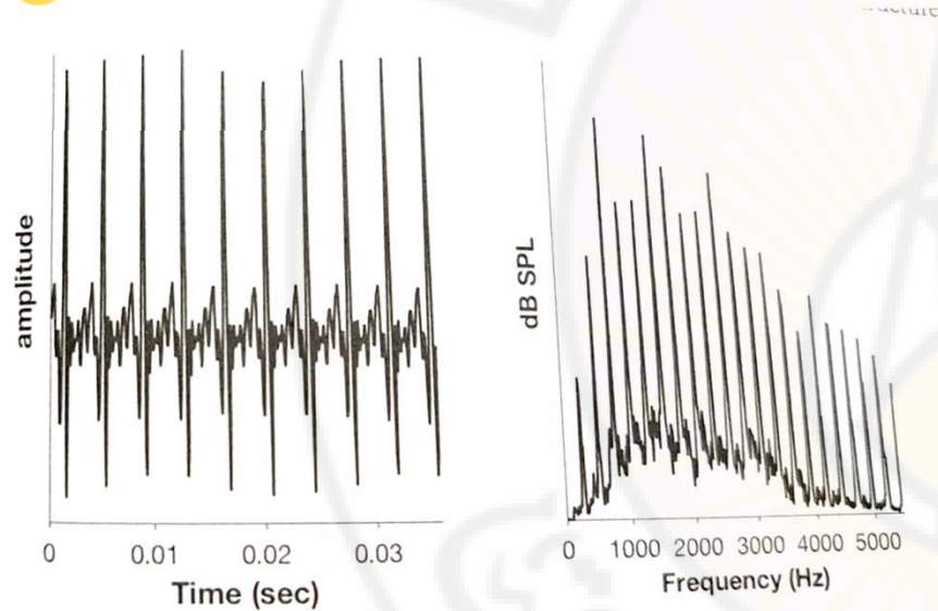
FIGURE 6-1. Waveform (left panel) and spectrum (right panel) of the musical note C4 ( f_0 = 261 Hz) played by a trumpet.
