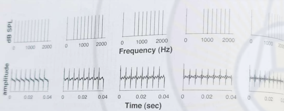
FIGURE 6-2. Illustration of the acoustic effect of removing low-frequency harmonics. Spectra (top panels) and waveforms (bottom panels) are shown. Low-frequency harmonics are progressively removed from a complex tone, illustrated by moving from the left panels to the right panels.
