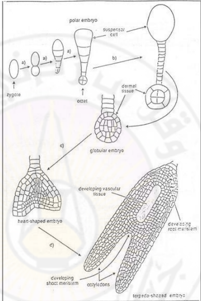
Figure -5 Major stages in the formation of the embryo. a) Formation of the polar embryo with a large suspensor cell at one end and an octet of cells at the other, b) division of octet to produce 16 cells in two layers, with subsequent development producing the globular embryo, c) uneven rates of cell division convert the globular-shaped embryo into a heart-shaped embryo and development continues to eventually produce the torpedo-shaped embryo shown in d). (Not drawn to scale).
