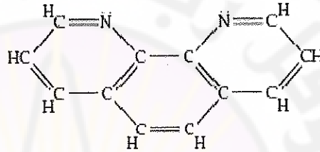
ortho-phenanthroline (phen)
