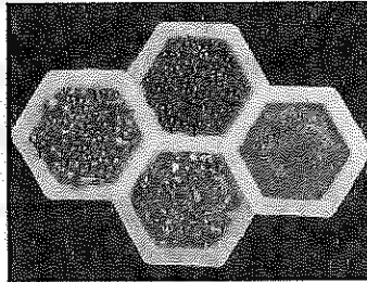
Group 4A: top, carbon (C); top, lead (Pb); right, tin (Sn); bottom, silicon (Si)
