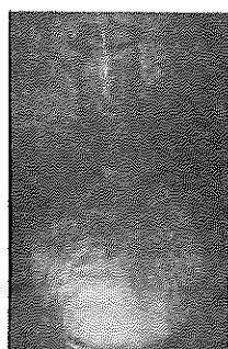
Group 5A: nitrogen ( \text{N}_2 )
