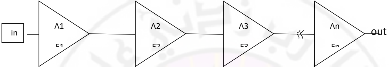
الشكل (13.3) Total noise figure
