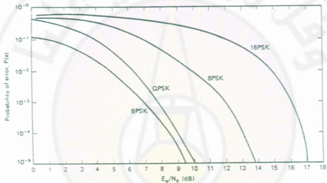
Probability of error P(e) versus E_b/N_0 ratio for various digital modulation schemes
