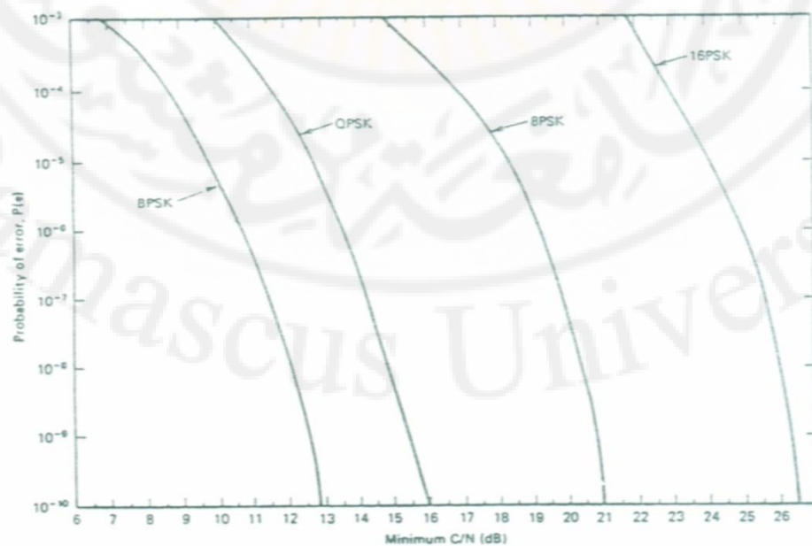
Probability of error P(e) versus C/N for various digital modulation schemes. (Bandwidth equals minimum double-sided Nyquist bandwidth.)
