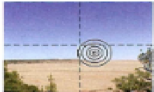
B Directional tuning of a neuron in the barn owl
