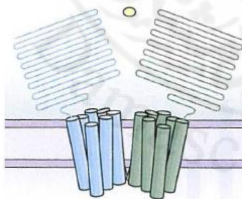
Sweet (T1R2 + T1R3)
