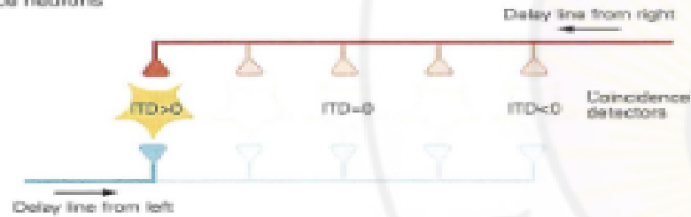
B Mapping of ITD onto array of neuronal coincidence neurons
