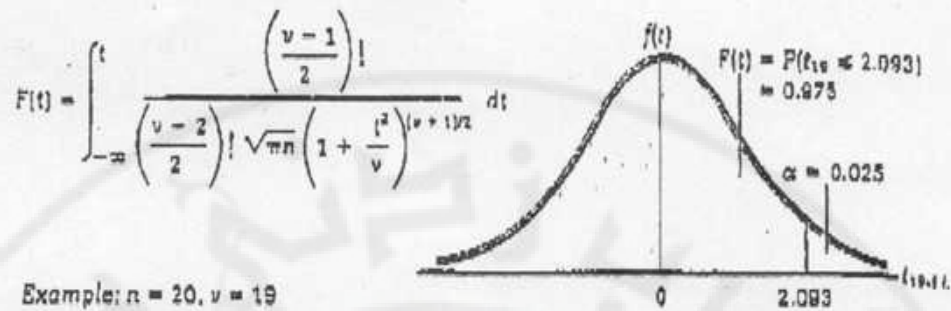
Cumulative t-distribution F(t)
