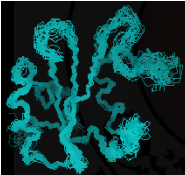
NMR models
